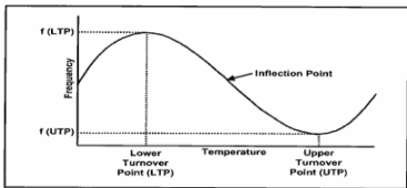
Frequency vs. Temperature Characteristics
